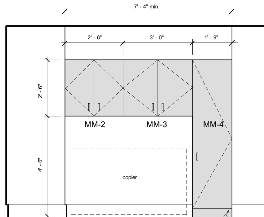
North Elevation at Copy 209D
